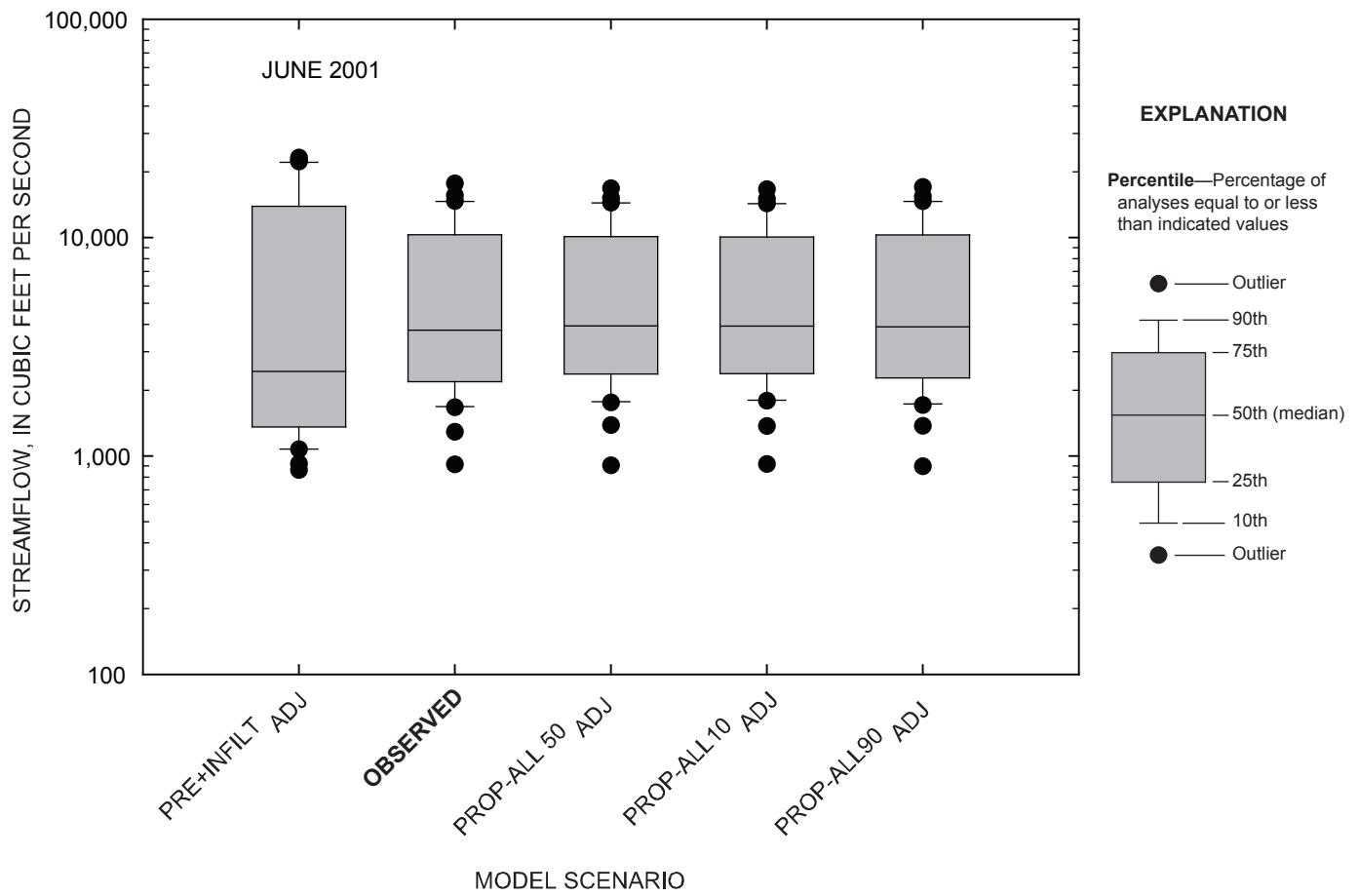
Figure 4-81. Comparison of daily streamflow for observed and simulated conditions at the Marais des Cygnes River near the Kansas-Missouri state line, Kansas, June 2001.
