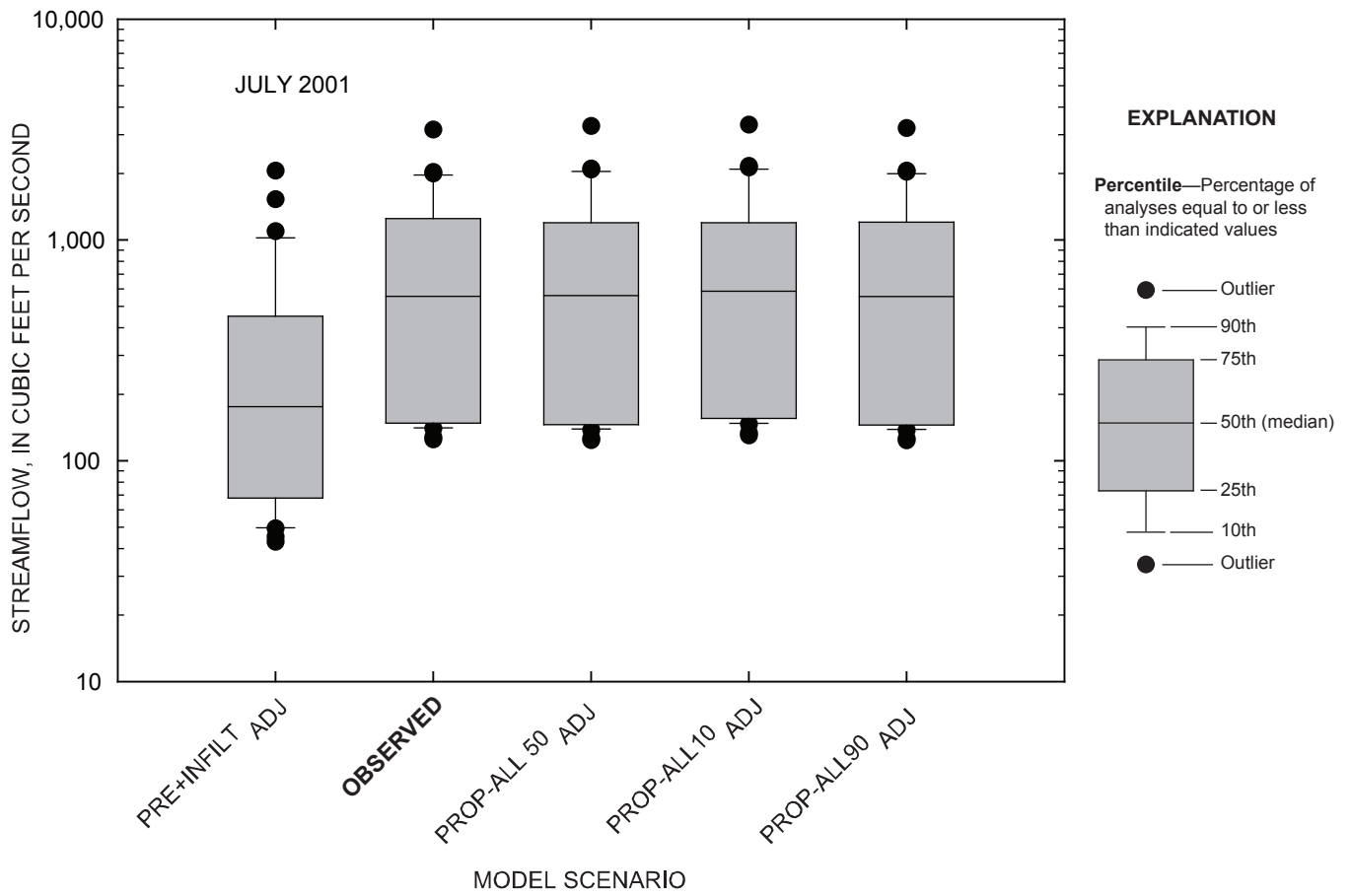
Figure 4-82. Comparison of daily streamflow for observed and simulated conditions at the Marais des Cygnes River near the Kansas-Missouri state line, Kansas, July 2001.
