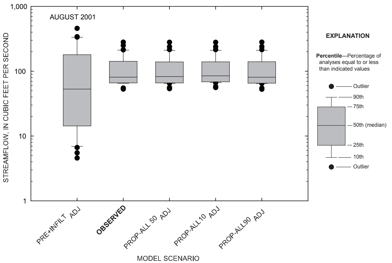
Figure 4-83. Comparison of daily streamflow for observed and simulated conditions at the Marais des Cygnes River near the Kansas-Missouri state line, Kansas, August 2001.
