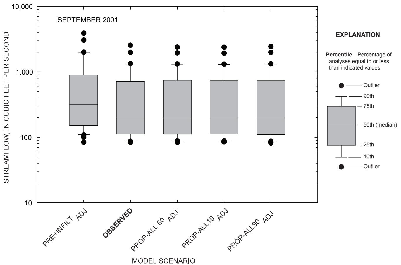
Figure 4-84. Comparison of daily streamflow for observed and simulated conditions at the Marais des Cygnes River near the Kansas-Missouri state line, Kansas, September 2001.
