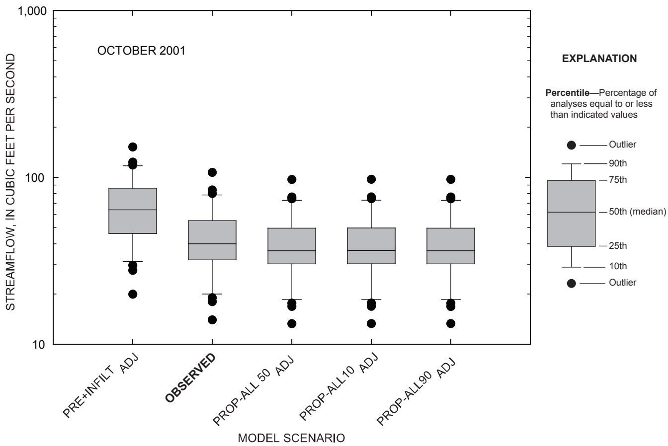
Figure 4-85. Comparison of daily streamflow for observed and simulated conditions at the Marais des Cygnes River near the Kansas-Missouri state line, Kansas, October 2001.
