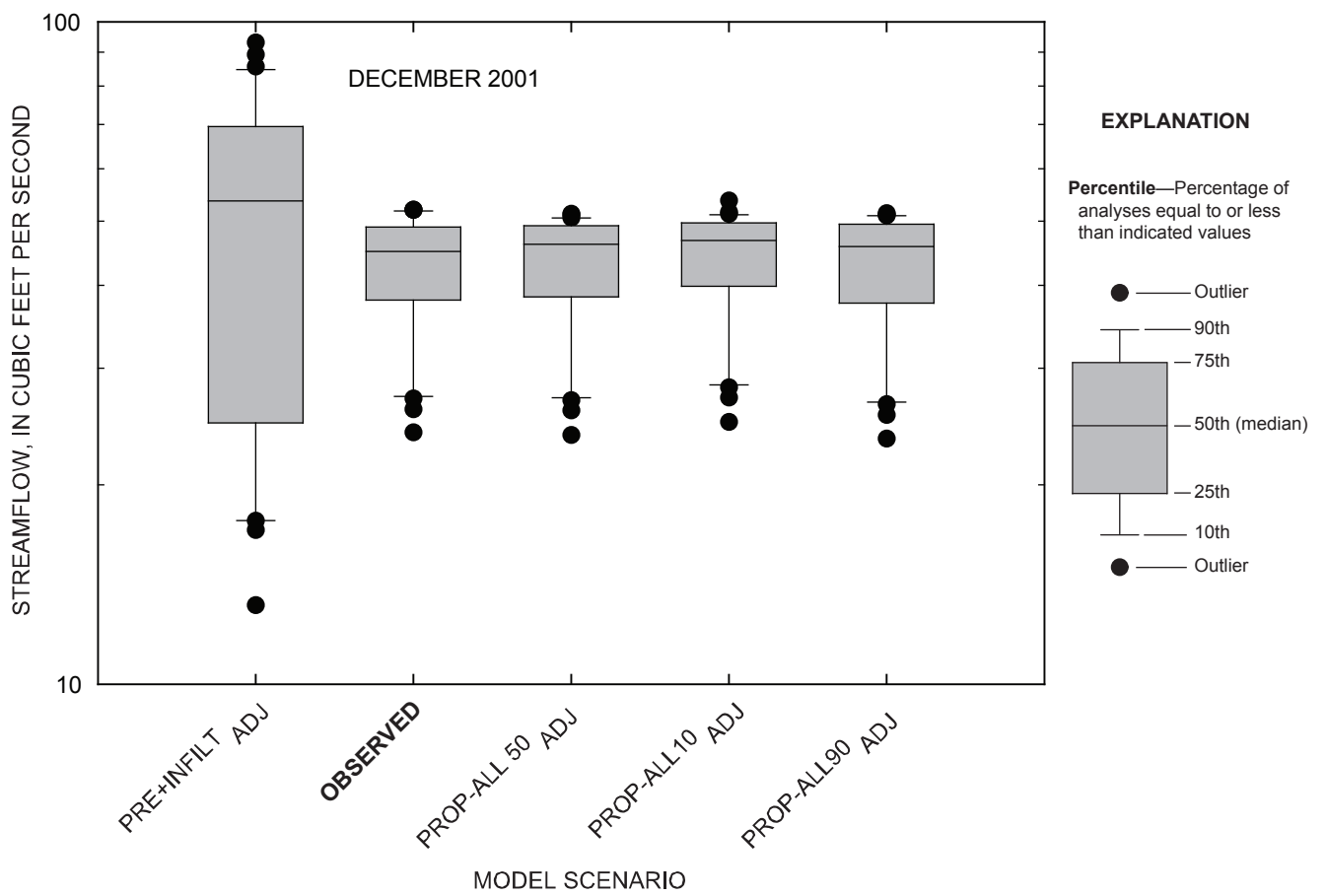
Figure 4-87. Comparison of daily streamflow for observed and simulated conditions at the Marais des Cygnes River near the Kansas-Missouri state line, Kansas, December 2001.
