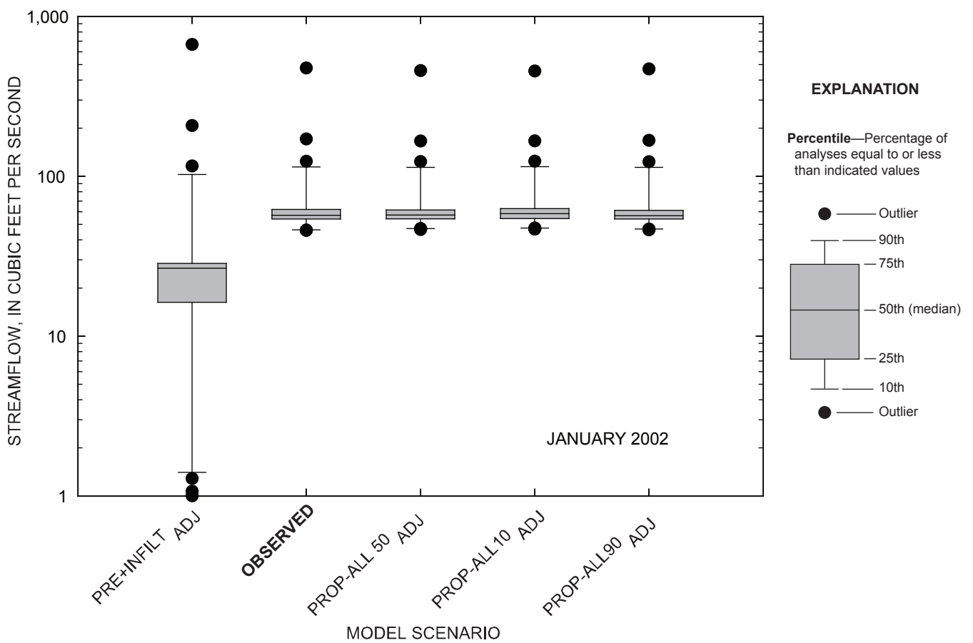
Figure 4-88. Comparison of daily streamflow for observed and simulated conditions at the Marais des Cygnes River near the Kansas-Missouri state line, Kansas, January 2002.
