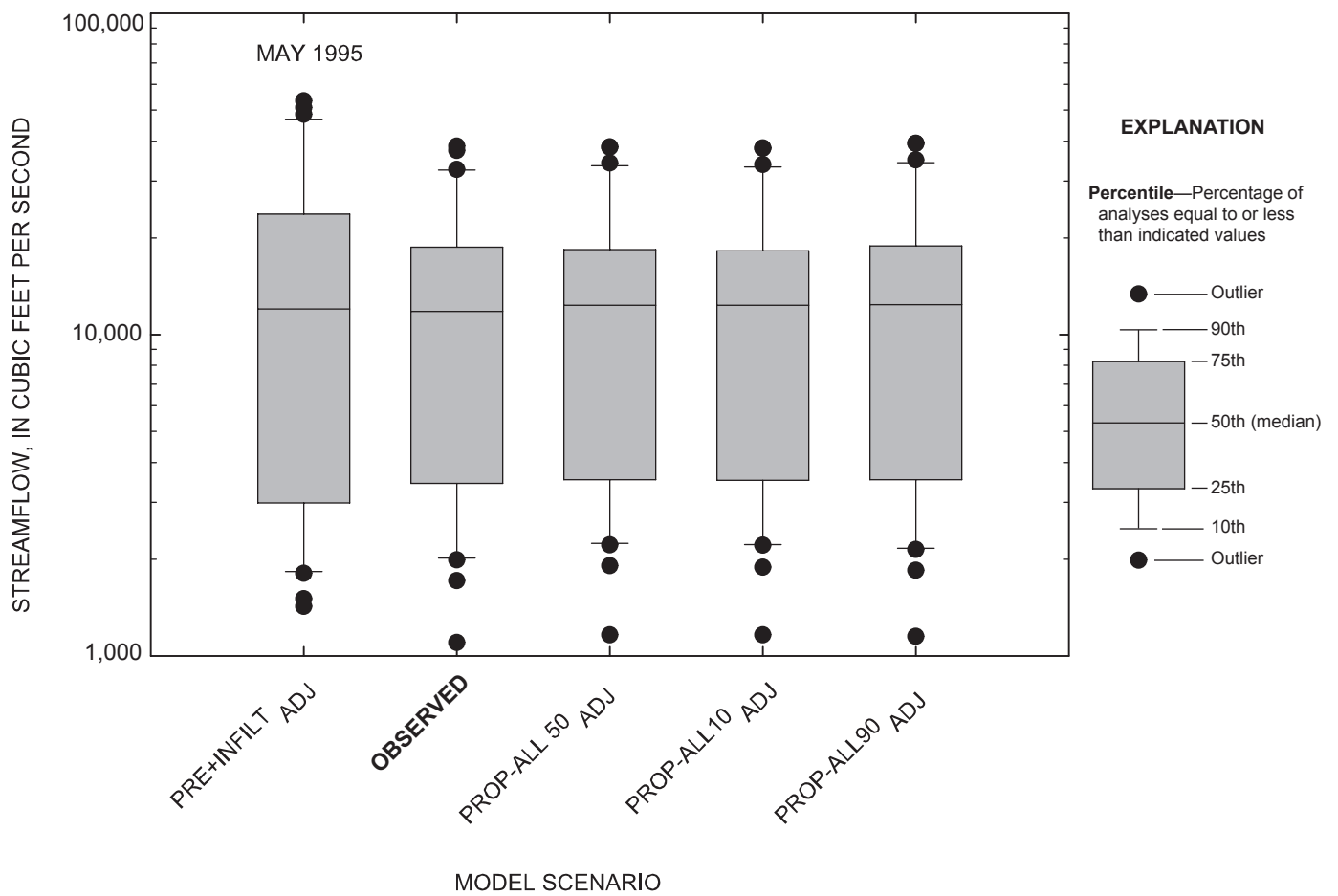
Figure 4-8. Comparison of daily streamflow for observed and simulated conditions at the Marais des Cygnes River near the Kansas-Missouri state line, Kansas, May 1995.
