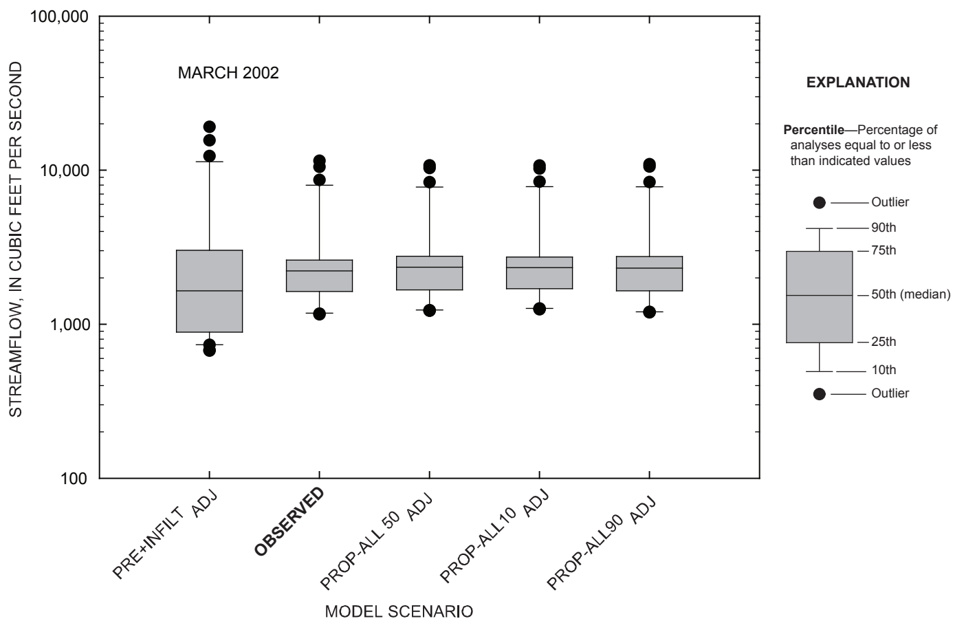
Figure 4-90. Comparison of daily streamflow for observed and simulated conditions at the Marais des Cygnes River near the Kansas-Missouri state line, Kansas, March 2002.
