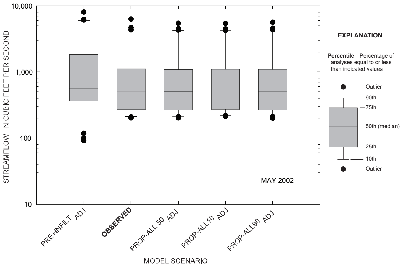
Figure 4-92. Comparison of daily streamflow for observed and simulated conditions at the Marais des Cygnes River near the Kansas-Missouri state line, Kansas, May 2002.
