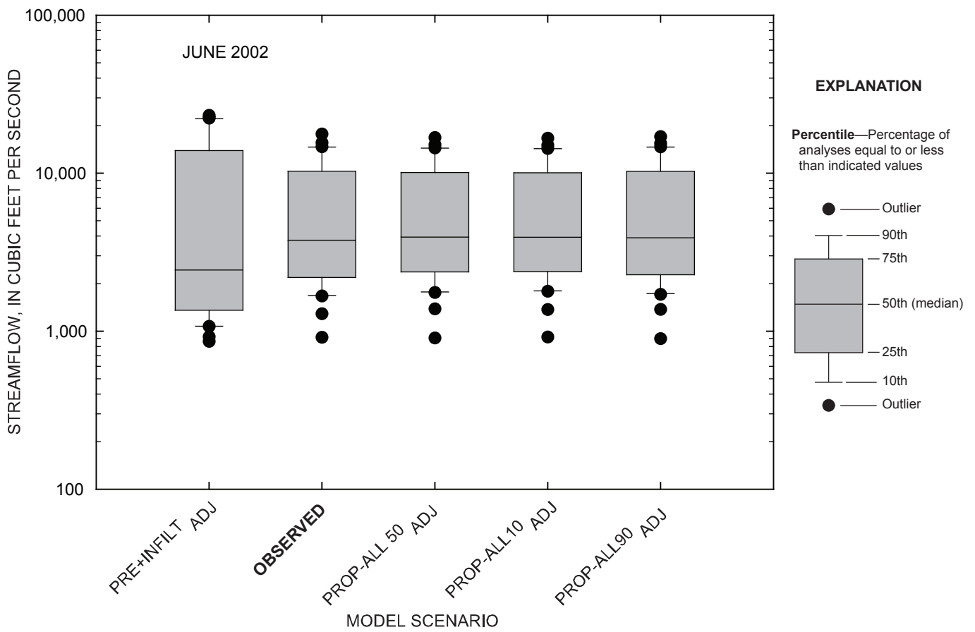
Figure 4-93. Comparison of daily streamflow for observed and simulated conditions at the Marais des Cygnes River near the Kansas-Missouri state line, Kansas, June 2002.
