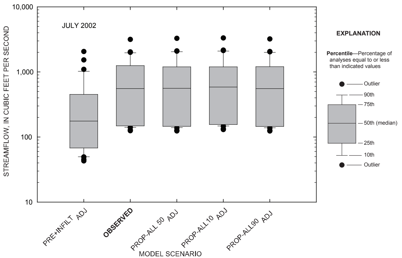
Figure 4-94. Comparison of daily streamflow for observed and simulated conditions at the Marais des Cygnes River near the Kansas-Missouri state line, Kansas, July 2002.
