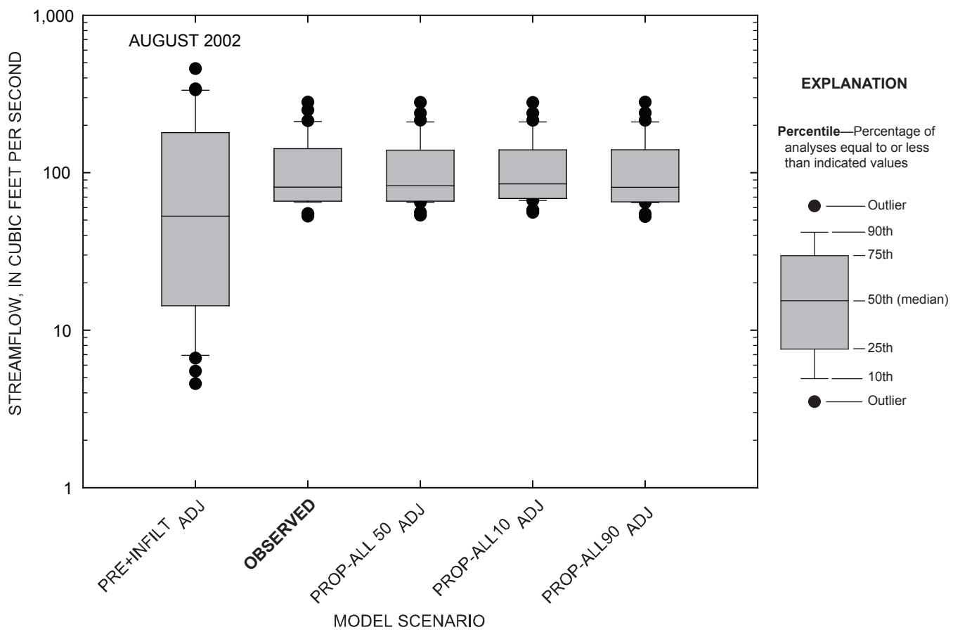
Figure 4-95. Comparison of daily streamflow for observed and simulated conditions at the Marais des Cygnes River near the Kansas-Missouri state line, Kansas, August 2002.
