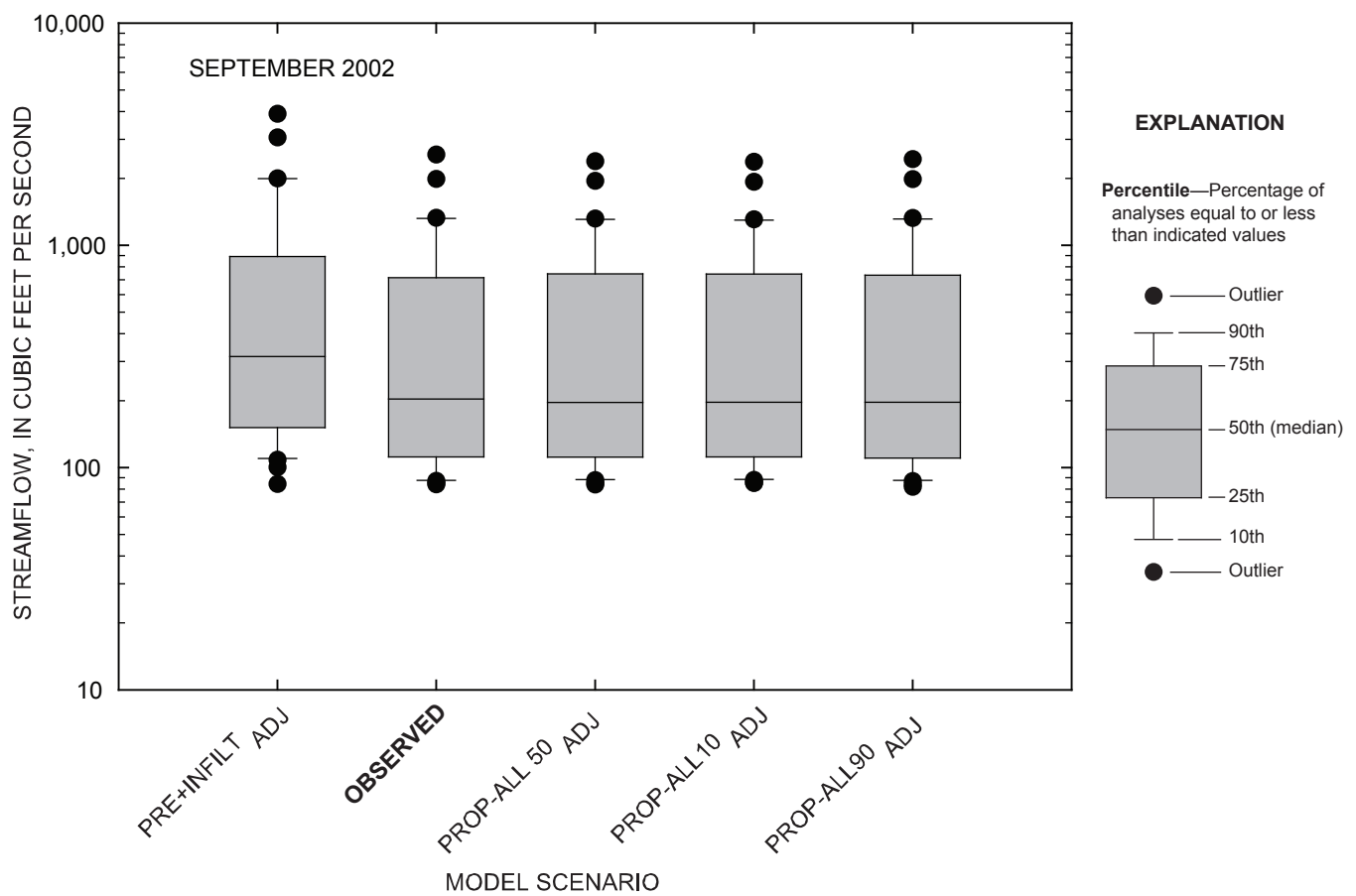
Figure 4-96. Comparison of daily streamflow for observed and simulated conditions at the Marais des Cygnes River near the Kansas-Missouri state line, Kansas, September 2002.
