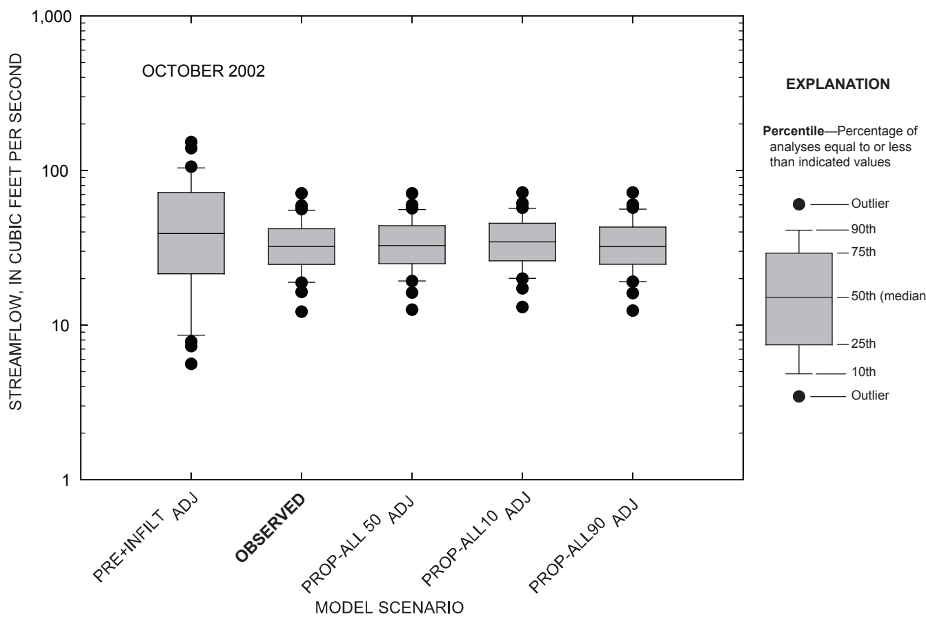
Figure 4-97. Comparison of daily streamflow for observed and simulated conditions at the Marais des Cygnes River near the Kansas-Missouri state line, Kansas, October 2002.
