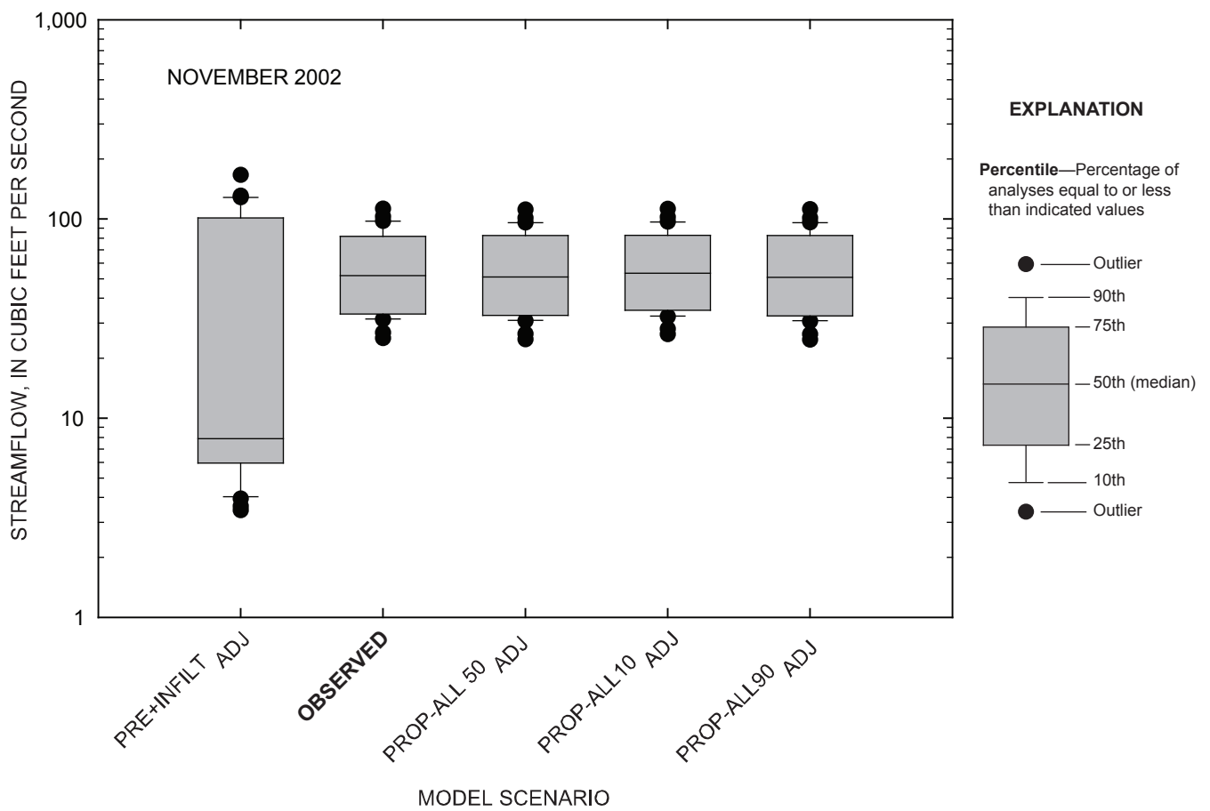
Figure 4-98. Comparison of daily streamflow for observed and simulated conditions at the Marais des Cygnes River near the Kansas-Missouri state line, Kansas, November 2002.
