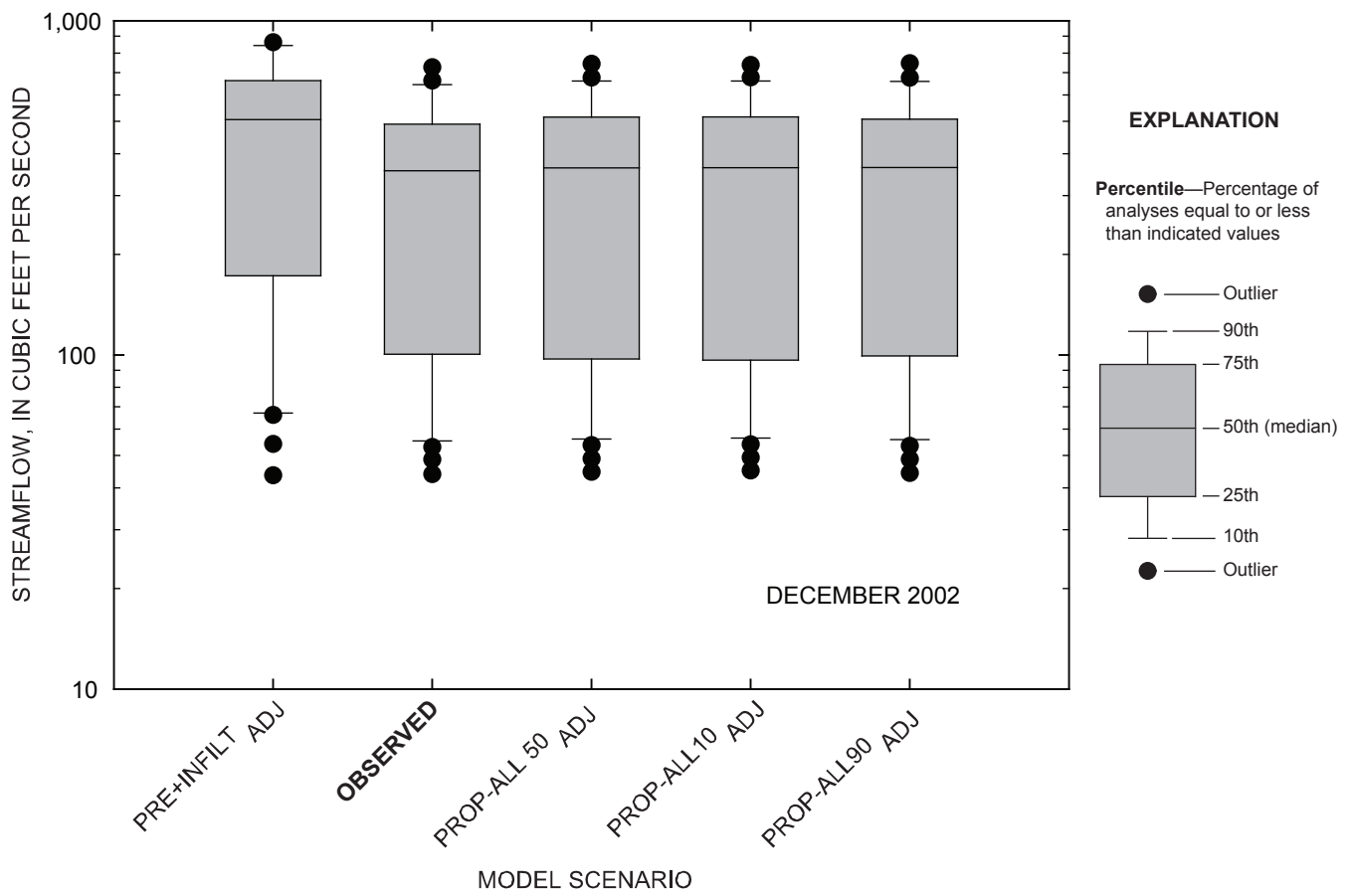
Figure 4-99. Comparison of daily streamflow for observed and simulated conditions at the Marais des Cygnes River near the Kansas-Missouri state line, Kansas, December 2002.
