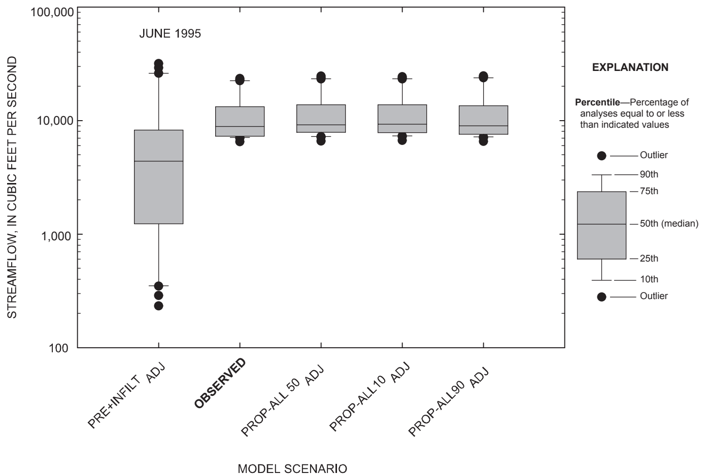
Figure 4-9. Comparison of daily streamflow for observed and simulated conditions at the Marais des Cygnes River near the Kansas-Missouri state line, Kansas, June 1995.
