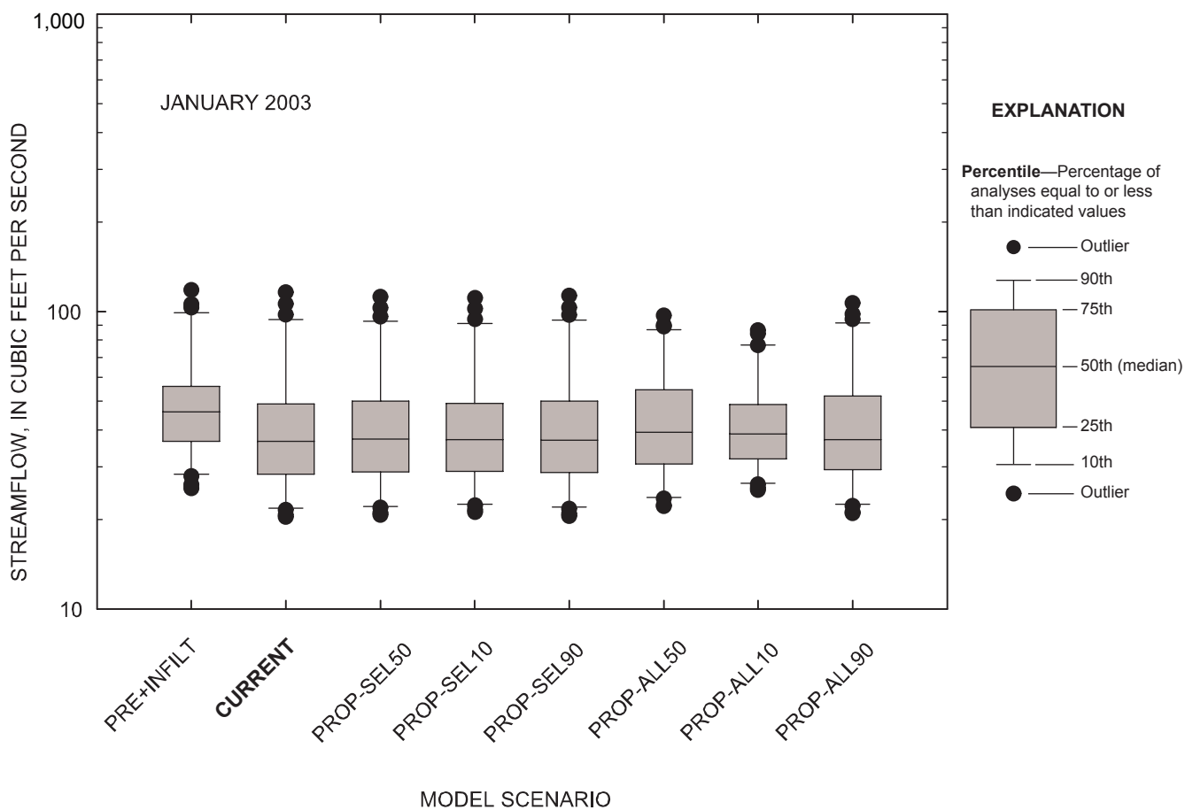
Figure 5-100. Comparison of daily streamflow for observed and simulated conditions at the Marmaton River near the Missouri-Kansas state line, Missouri, January 2003.
