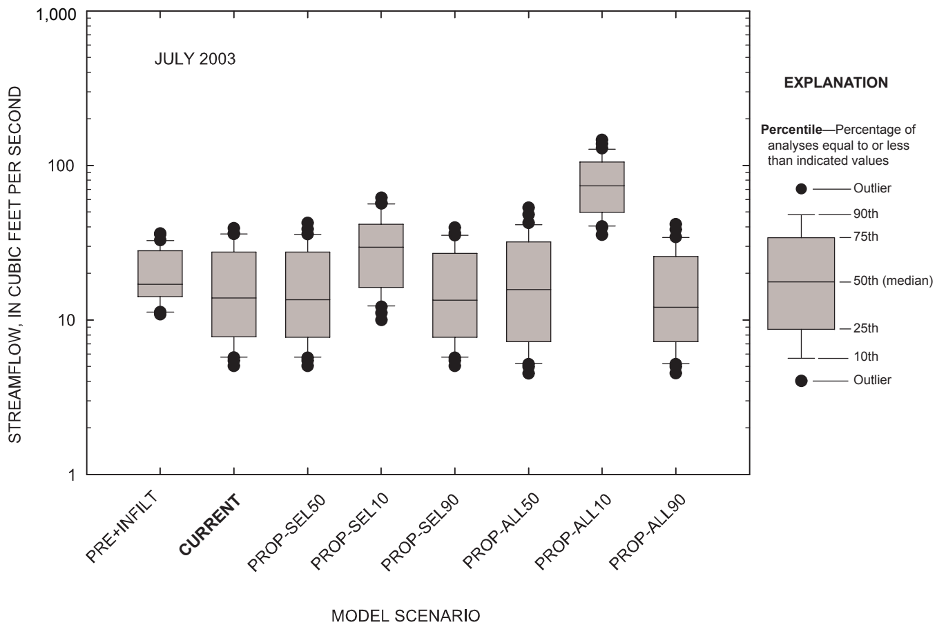
Figure 5-106. Comparison of daily streamflow for observed and simulated conditions at the Marmaton River near the Missouri-Kansas state line, Missouri, July 2003.
