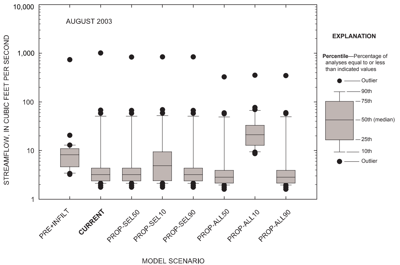
Figure 5-107. Comparison of daily streamflow for observed and simulated conditions at the Marmaton River near the Missouri-Kansas state line, Missouri, August 2003.
