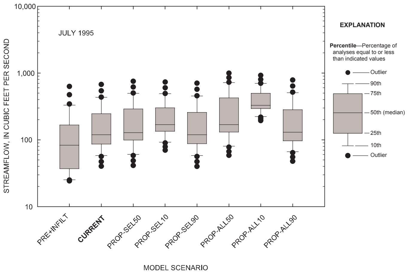
Figure 5-10. Comparison of daily streamflow for observed and simulated conditions at the Marmaton River near the Missouri-Kansas state line, Missouri, July 1995.
