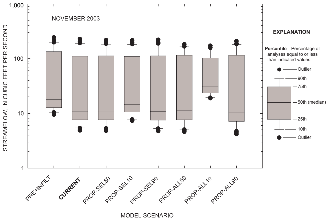
Figure 5-110. Comparison of daily streamflow for observed and simulated conditions at the Marmaton River near the Missouri-Kansas state line, Missouri, November 2003.
