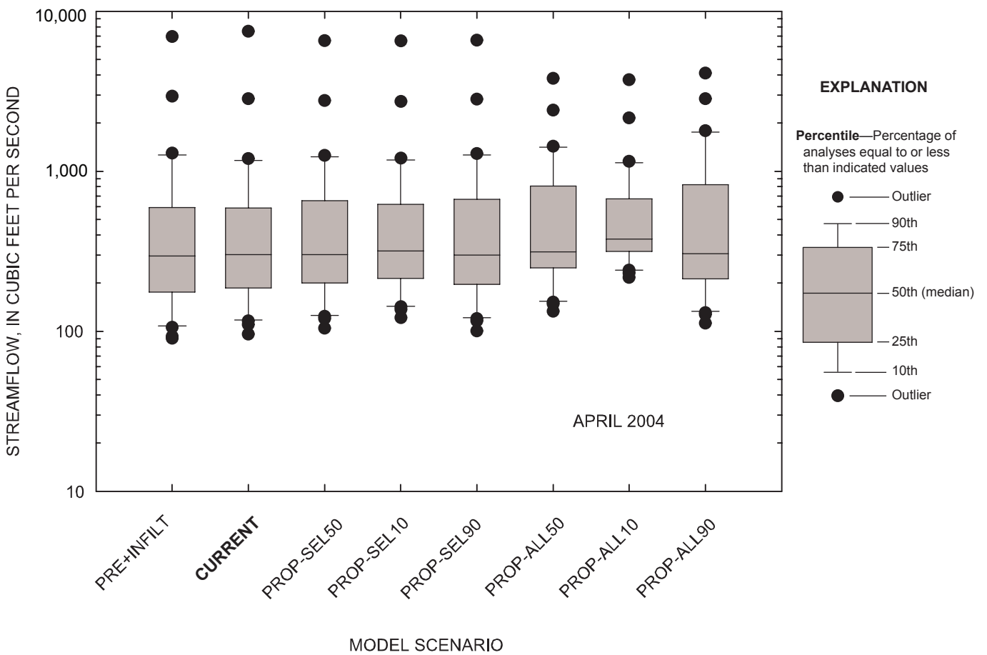
Figure 5-115. Comparison of daily streamflow for observed and simulated conditions at the Marmaton River near the Missouri-Kansas state line, Missouri, April 2004.
