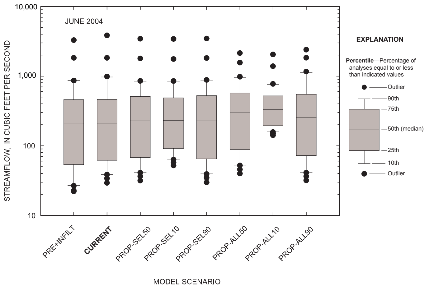
Figure 5-117. Comparison of daily streamflow for observed and simulated conditions at the Marmaton River near the Missouri-Kansas state line, Missouri, June 2004.
