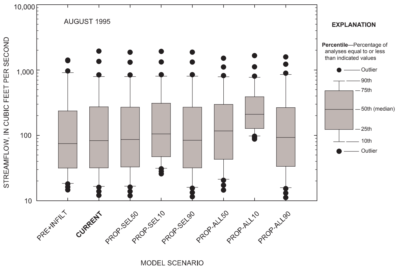
Figure 5-11. Comparison of daily streamflow for observed and simulated conditions at the Marmaton River near the Missouri-Kansas state line, Missouri, August 1995.
