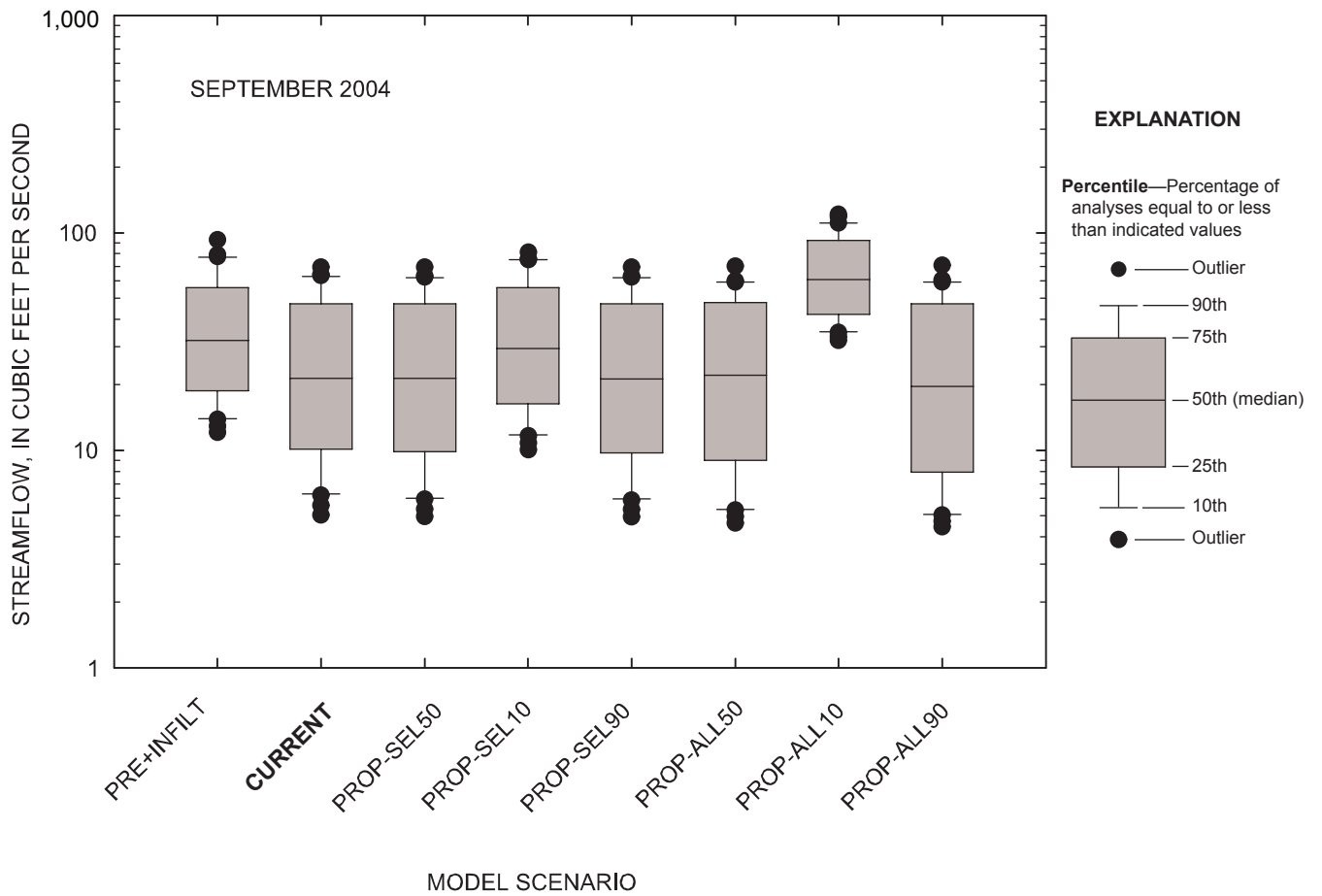
Figure 5-120. Comparison of daily streamflow for observed and simulated conditions at the Marmaton River near the Missouri-Kansas state line, Missouri, September 2004.
