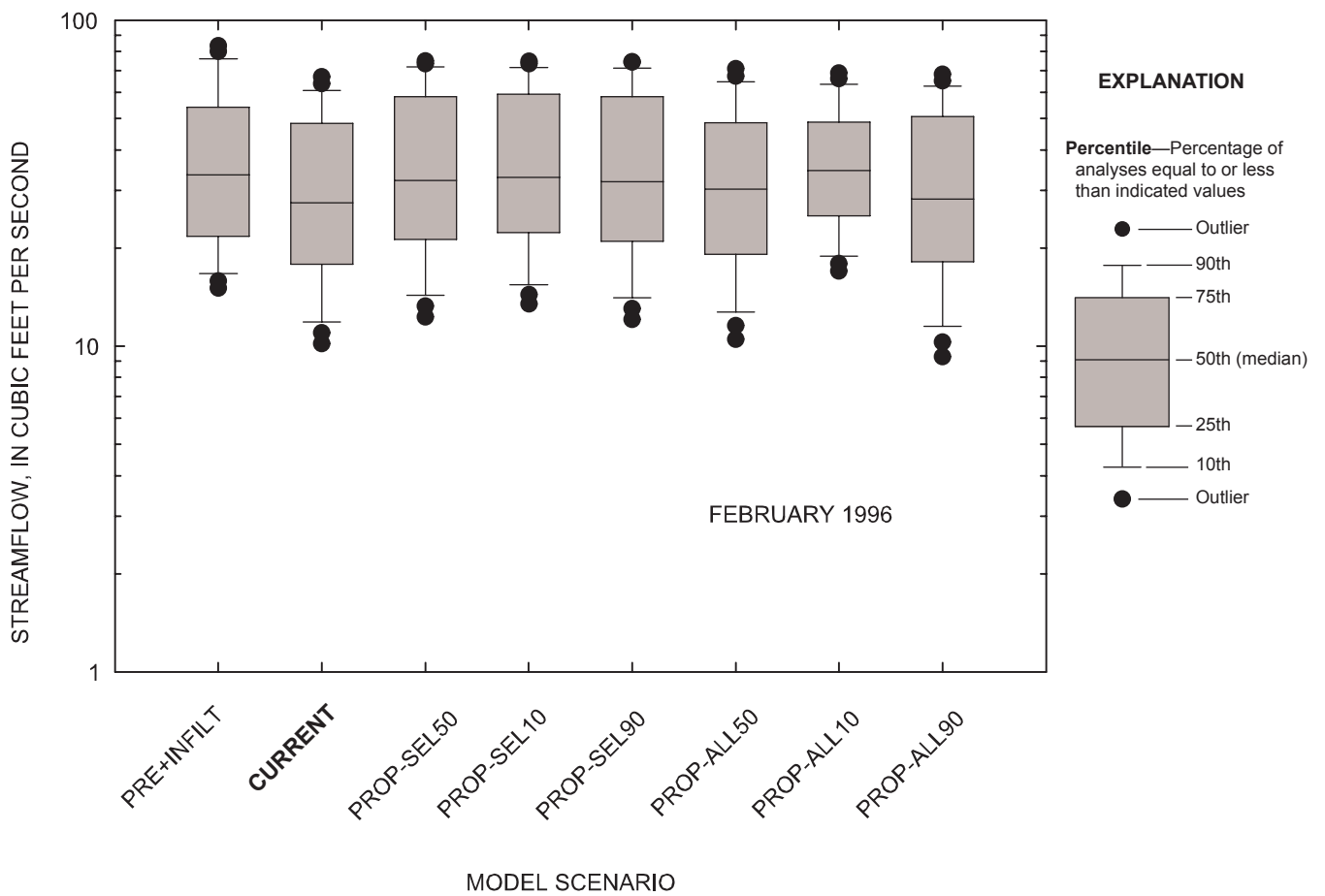
Figure 5-17. Comparison of daily streamflow for observed and simulated conditions at the Marmaton River near the Missouri-Kansas state line, Missouri, February 1996.
