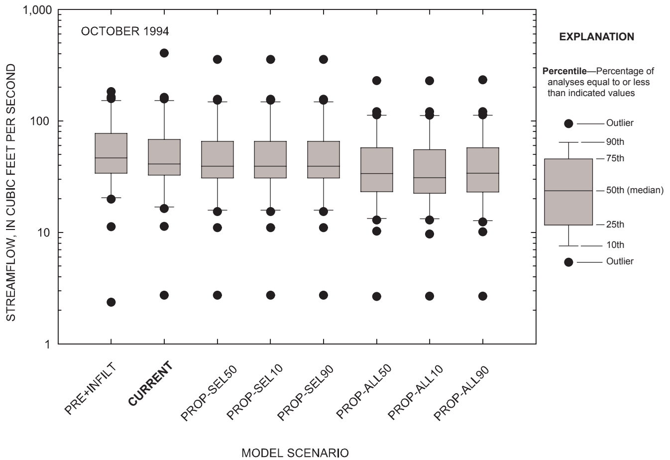
Figure 5-1. Comparison of daily streamflow for observed and simulated conditions at the Marmaton River near the Missouri-Kansas state line, Missouri, October 1994.
