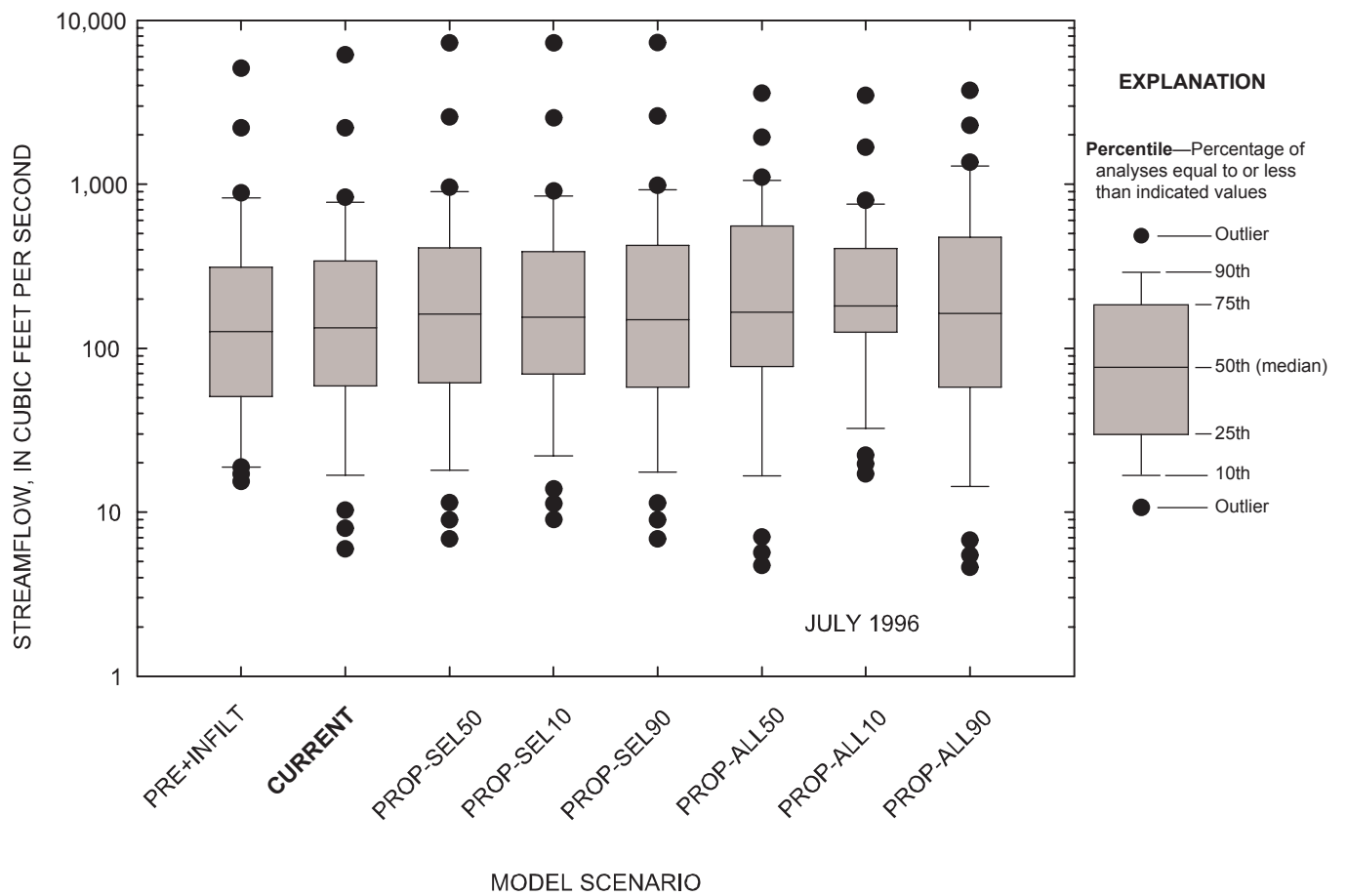
Figure 5-22. Comparison of daily streamflow for observed and simulated conditions at the Marmaton River near the Missouri-Kansas state line, Missouri, July 1996.
