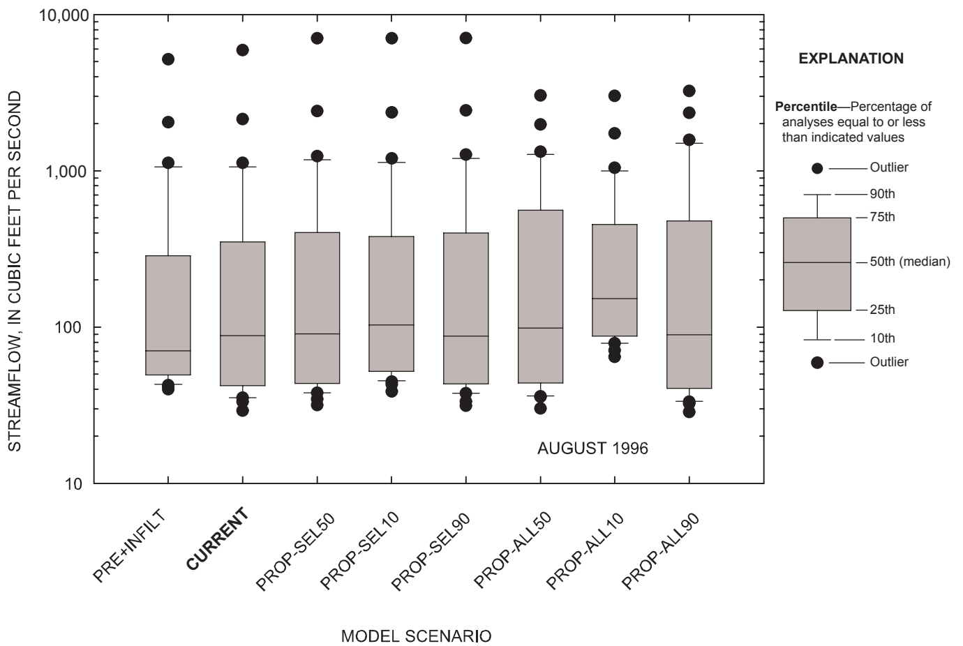
Figure 5-23. Comparison of daily streamflow for observed and simulated conditions at the Marmaton River near the Missouri-Kansas state line, Missouri, August 1996.
