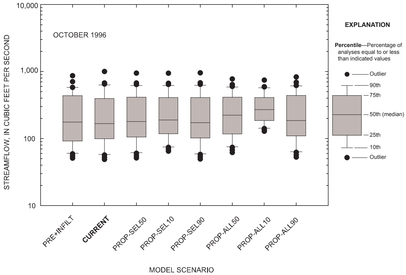
Figure 5-25. Comparison of daily streamflow for observed and simulated conditions at the Marmaton River near the Missouri-Kansas state line, Missouri, October 1996.
