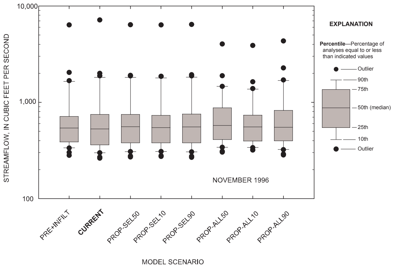
Figure 5-26. Comparison of daily streamflow for observed and simulated conditions at the Marmaton River near the Missouri-Kansas state line, Missouri, November 1996.
