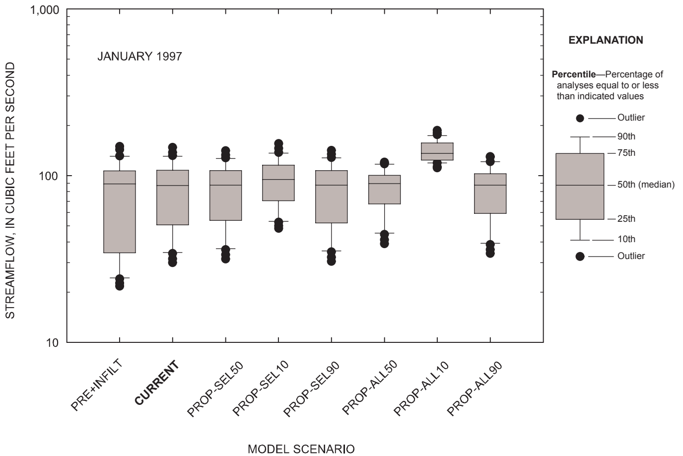
Figure 5-28. Comparison of daily streamflow for observed and simulated conditions at the Marmaton River near the Missouri-Kansas state line, Missouri, January 1997.
