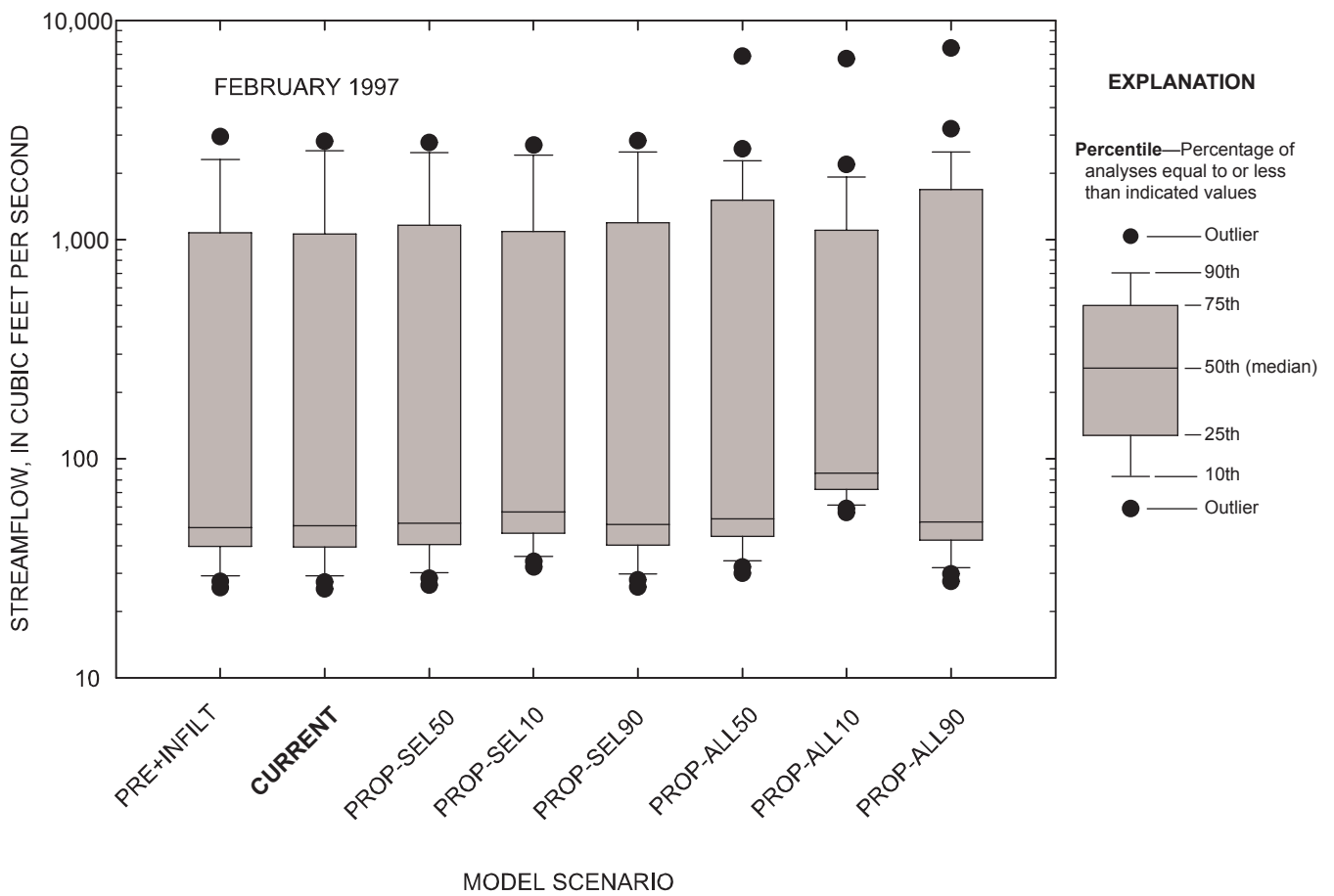
Figure 5-29. Comparison of daily streamflow for observed and simulated conditions at the Marmaton River near the Missouri-Kansas state line, Missouri, February 1997.
