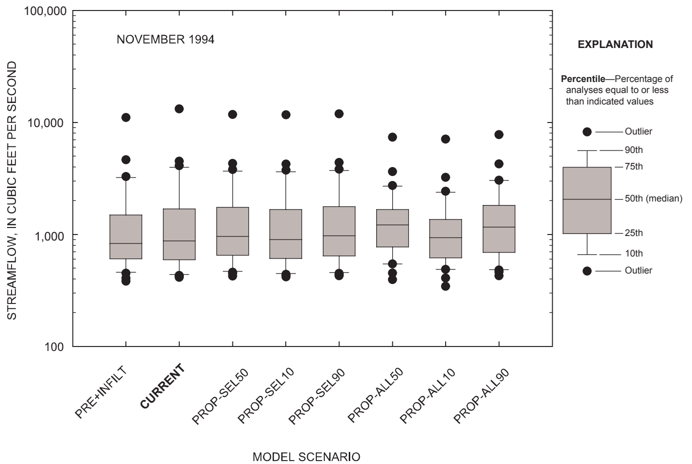
Figure 5-2. Comparison of daily streamflow for observed and simulated conditions at the Marmaton River near the Missouri-Kansas state line, Missouri, November 1994.
