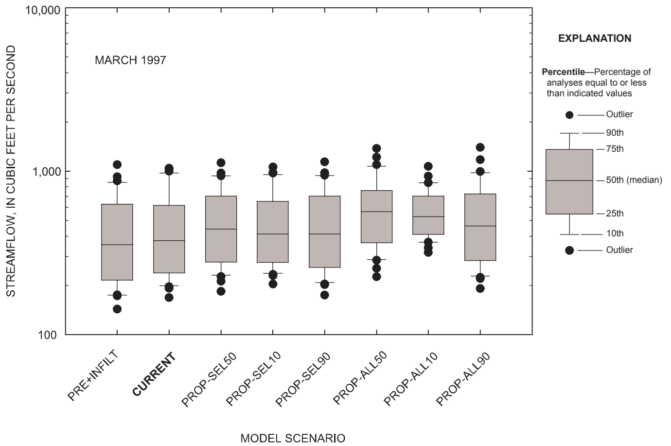
Figure 5-30. Comparison of daily streamflow for observed and simulated conditions at the Marmaton River near the Missouri-Kansas state line, Missouri, March 1997.
