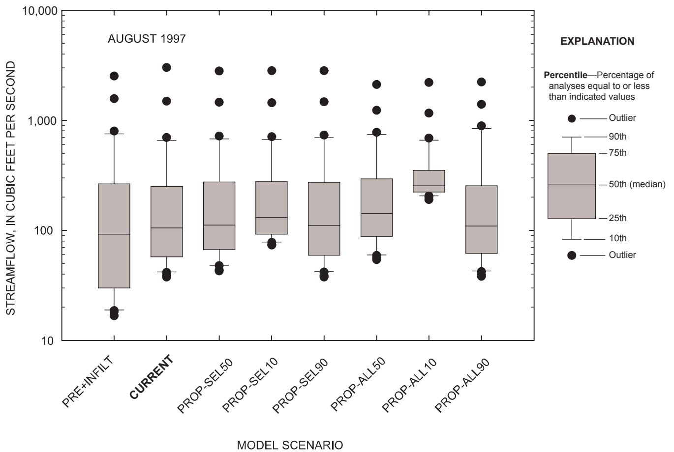
Figure 5-35. Comparison of daily streamflow for observed and simulated conditions at the Marmaton River near the Missouri-Kansas state line, Missouri, August 1997.
