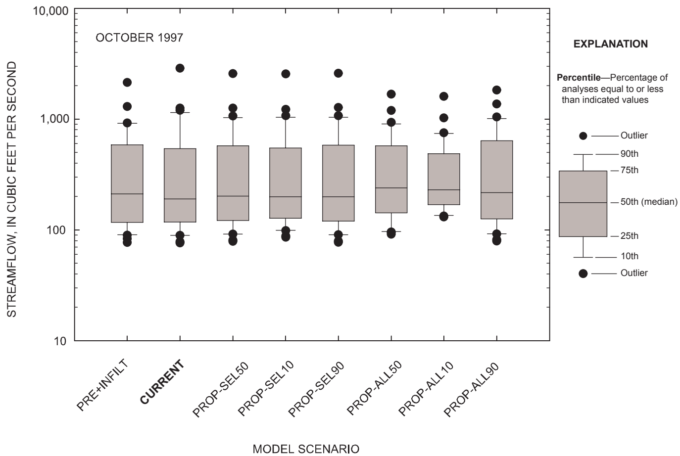
Figure 5-37. Comparison of daily streamflow for observed and simulated conditions at the Marmaton River near the Missouri-Kansas state line, Missouri, October 1997.
