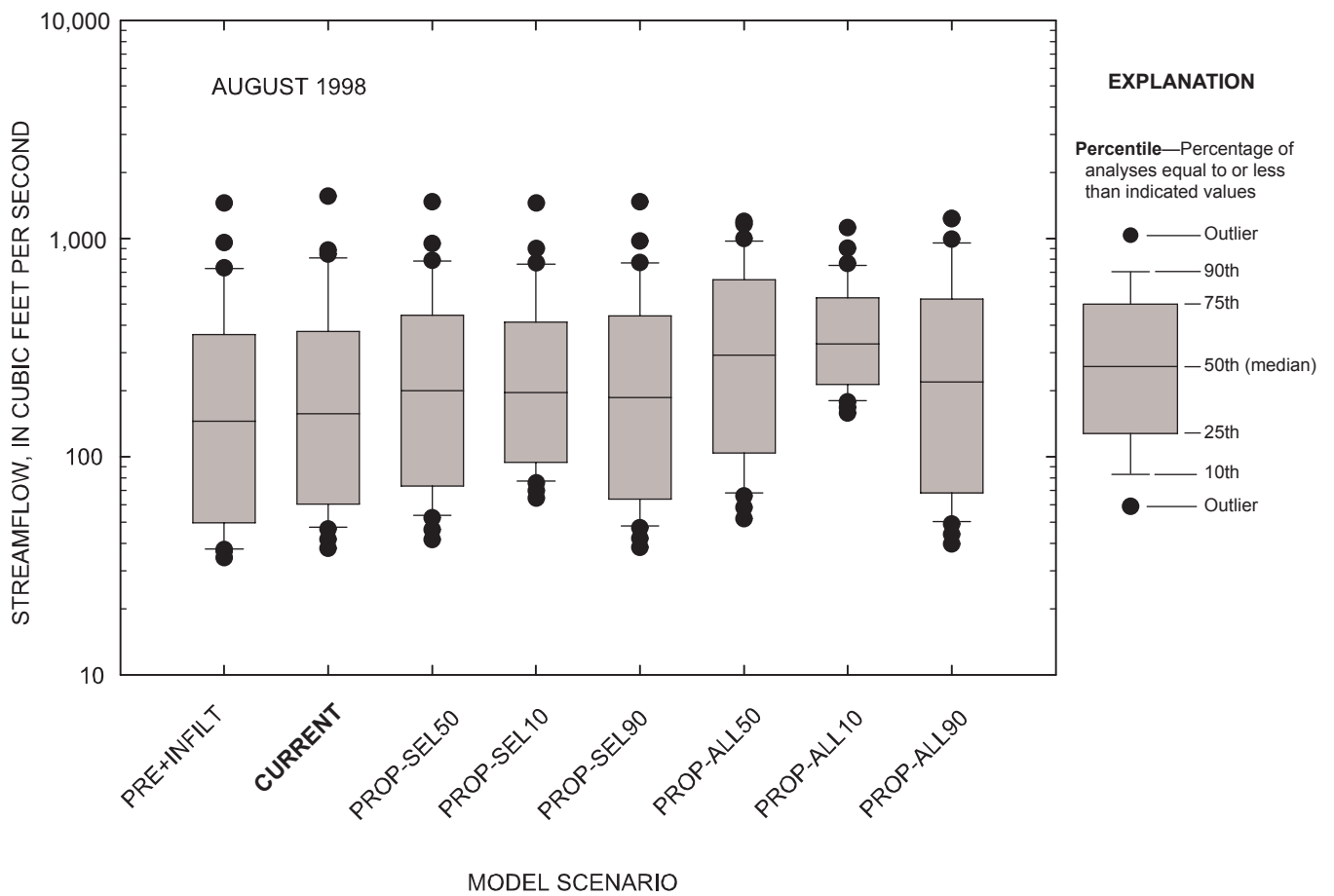
Figure 5-47. Comparison of daily streamflow for observed and simulated conditions at the Marmaton River near the Missouri-Kansas state line, Missouri, August 1998.
