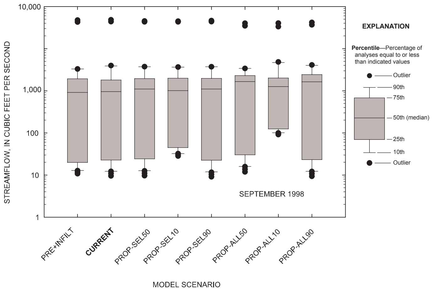
Figure 5-48. Comparison of daily streamflow for observed and simulated conditions at the Marmaton River near the Missouri-Kansas state line, Missouri, September 1998.
