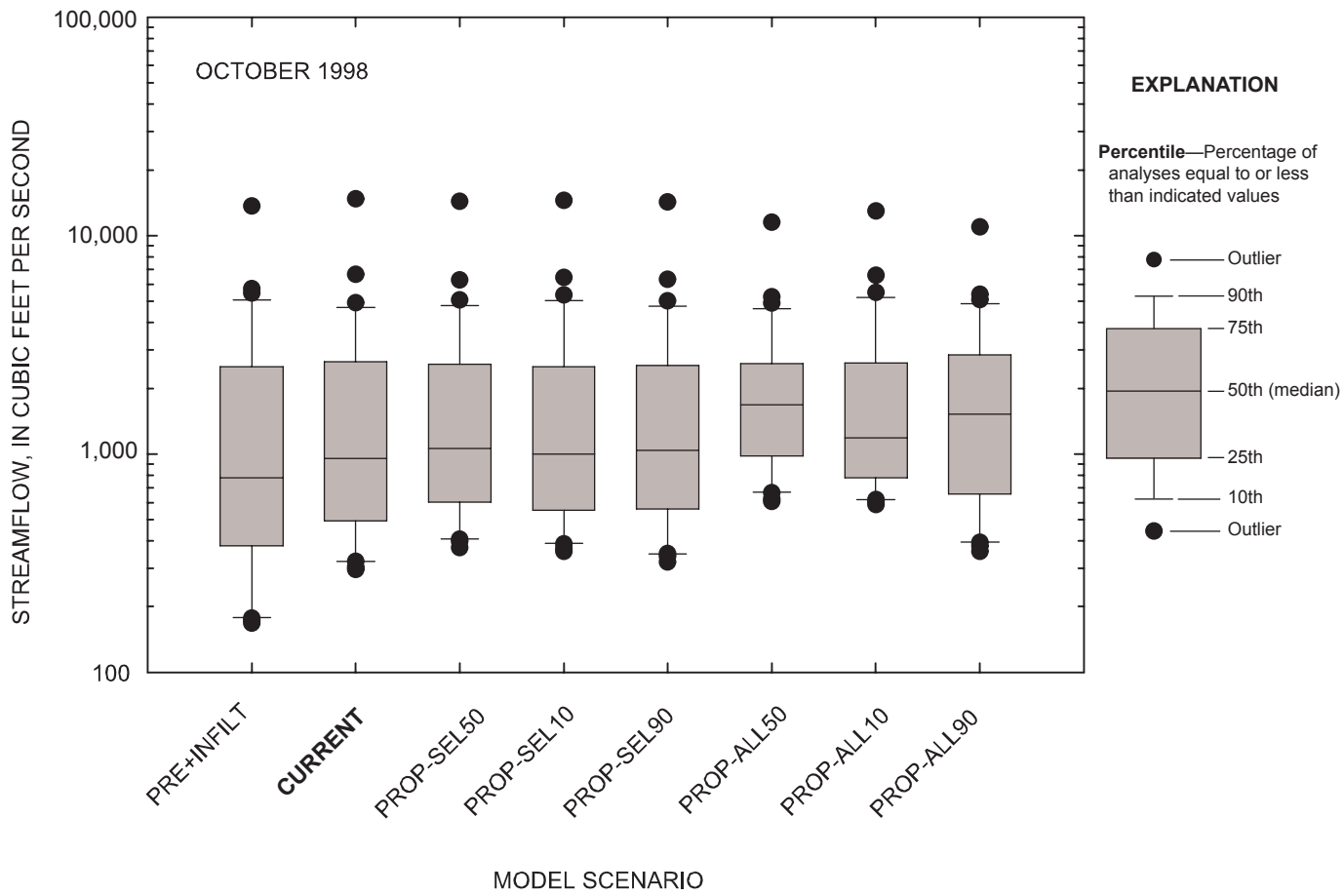
Figure 5-49. Comparison of daily streamflow for observed and simulated conditions at the Marmaton River near the Missouri-Kansas state line, Missouri, October 1998.
