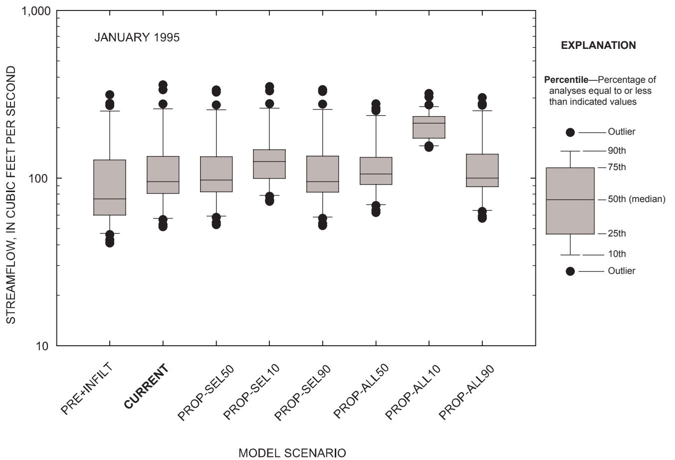
Figure 5-4. Comparison of daily streamflow for observed and simulated conditions at the Marmaton River near the Missouri-Kansas state line, Missouri, January 1995.
