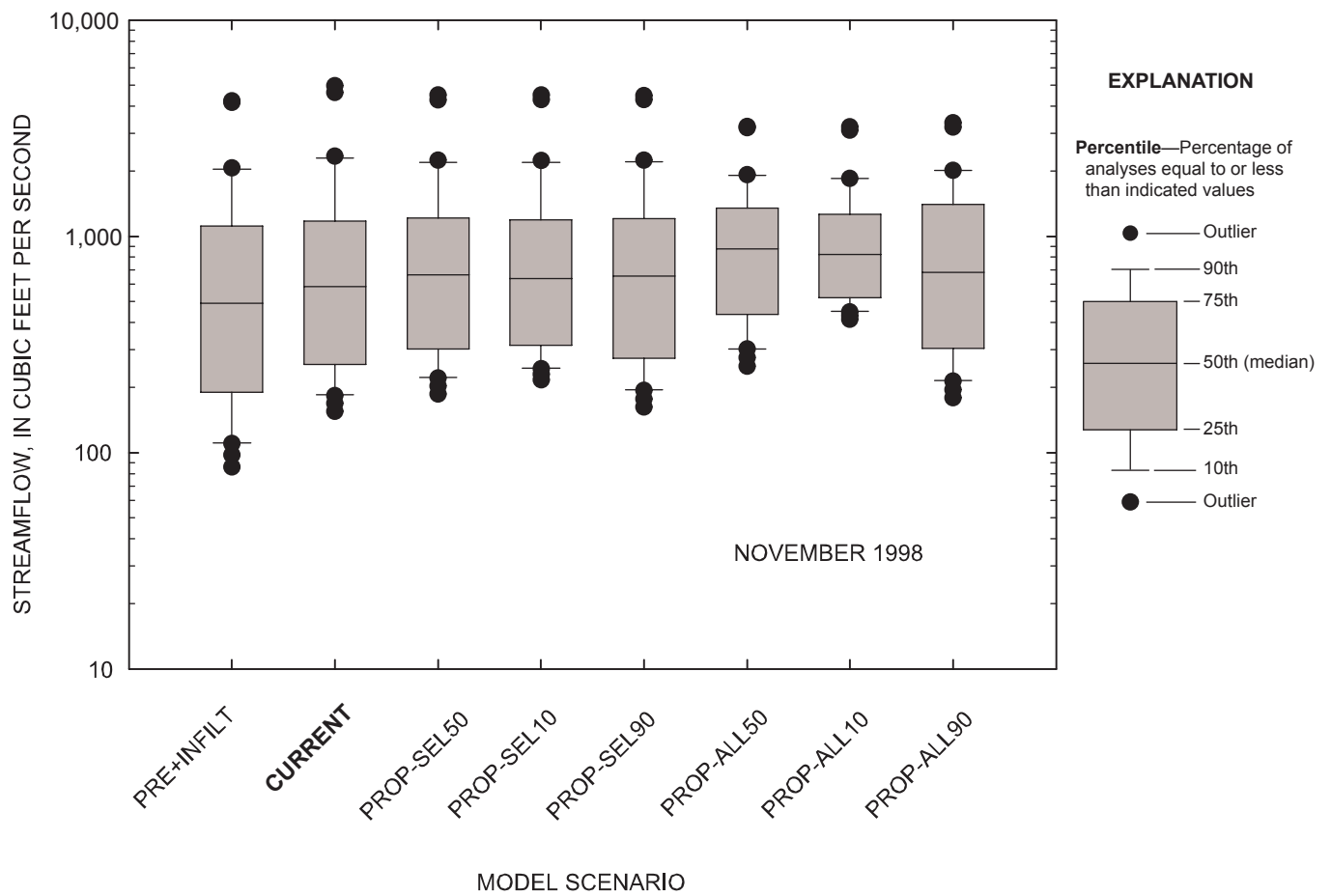
Figure 5-50. Comparison of daily streamflow for observed and simulated conditions at the Marmaton River near the Missouri-Kansas state line, Missouri, November 1998.
