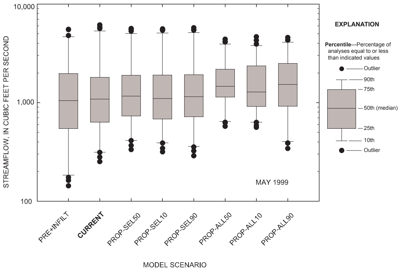
Figure 5-56. Comparison of daily streamflow for observed and simulated conditions at the Marmaton River near the Missouri-Kansas state line, Missouri, May 1999.
