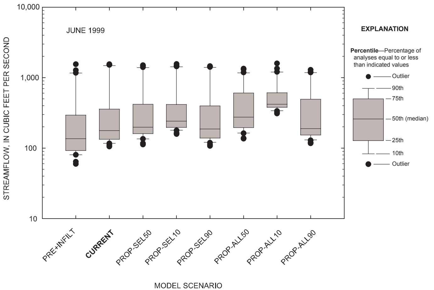
Figure 5-57. Comparison of daily streamflow for observed and simulated conditions at the Marmaton River near the Missouri-Kansas state line, Missouri, June 1999.
