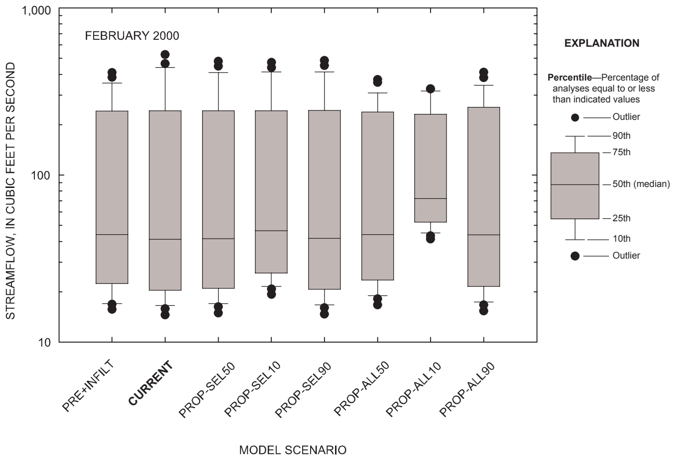
Figure 5-65. Comparison of daily streamflow for observed and simulated conditions at the Marmaton River near the Missouri-Kansas state line, Missouri, February 2000.
