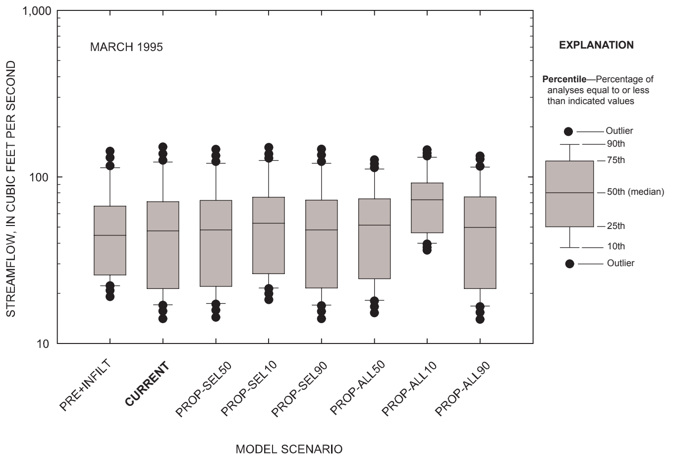
Figure 5-6. Comparison of daily streamflow for observed and simulated conditions at the Marmaton River near the Missouri-Kansas state line, Missouri, March 1995.
