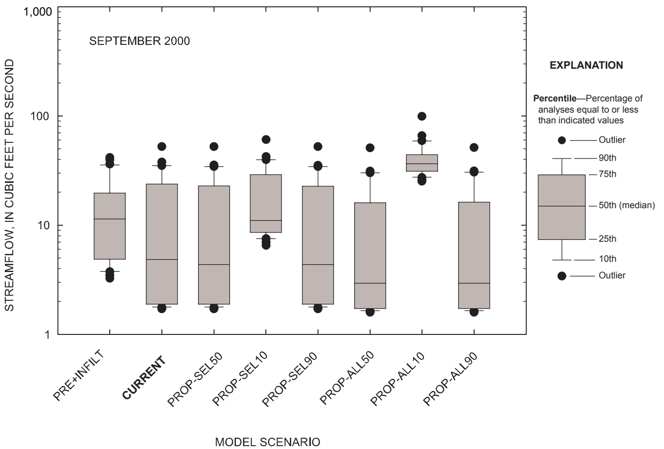
Figure 5-72. Comparison of daily streamflow for observed and simulated conditions at the Marmaton River near the Missouri-Kansas state line, Missouri, September 2000.
