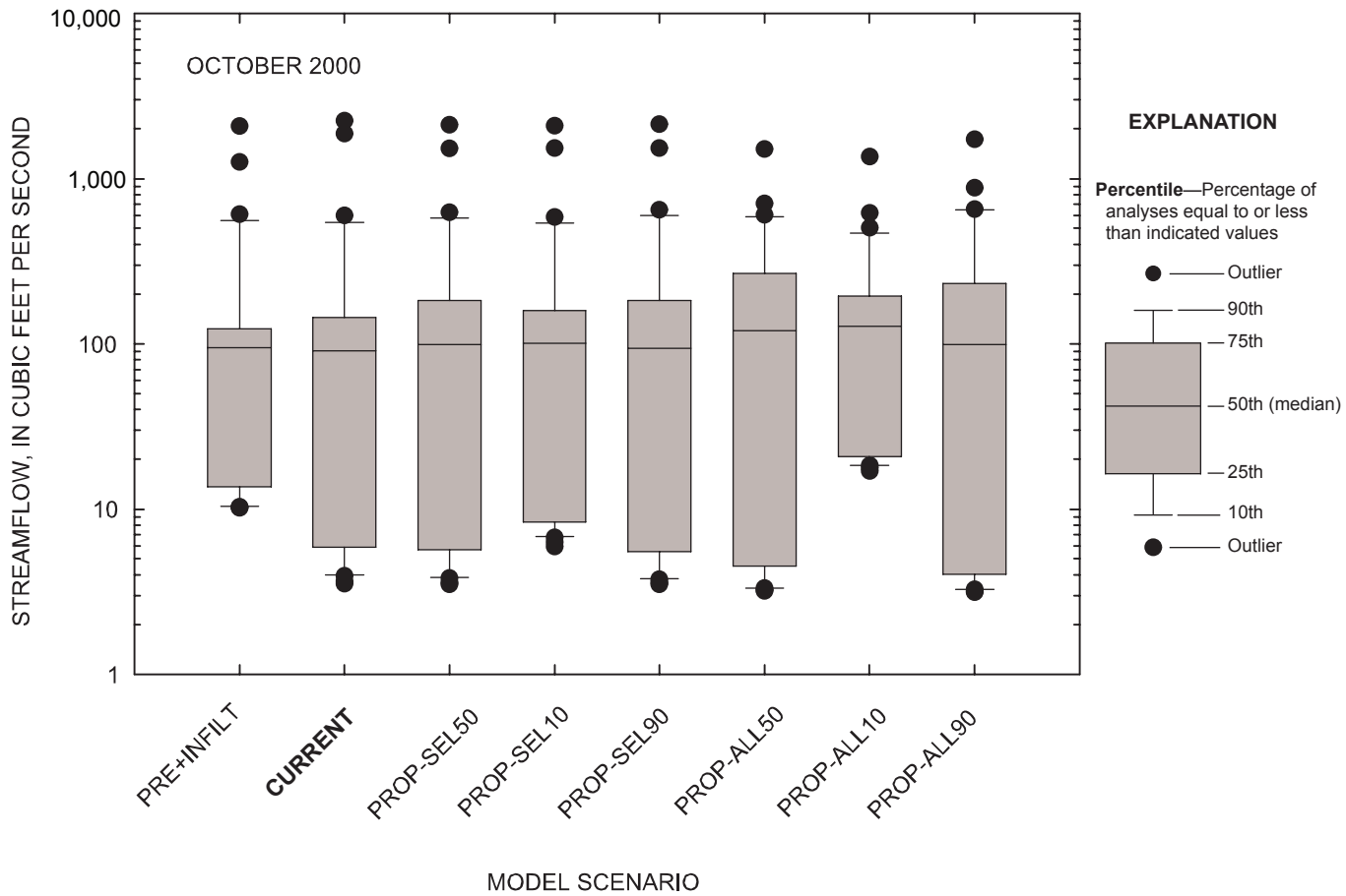
Figure 5-73. Comparison of daily streamflow for observed and simulated conditions at the Marmaton River near the Missouri-Kansas state line, Missouri, October 2000.
